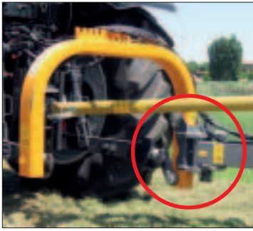
Floating frame: the joint pin on tractor side allows the head system to follow the ground, protecting the arms structure of the parallelogram.
